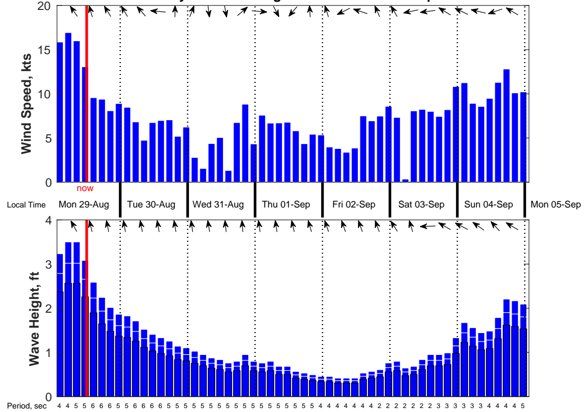
Wind & Wave Forecast for TABS Buoy R from 29-Aug-2022 01:00:00 to 04-Sep-2022 22:00:00
